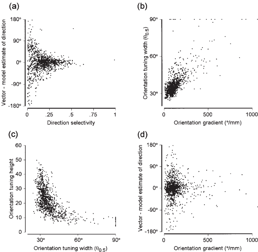
Figure 3. ( a–c ) Relationships between selected map parameters. Each graph shows data from 1000 points taken at random (avoiding duplication) from dataset 1. Results from other maps were qualitatively similar except for ( c ) where in datasets 2 and 3 fewer points with orientation tuning height values greater than 30 were present
